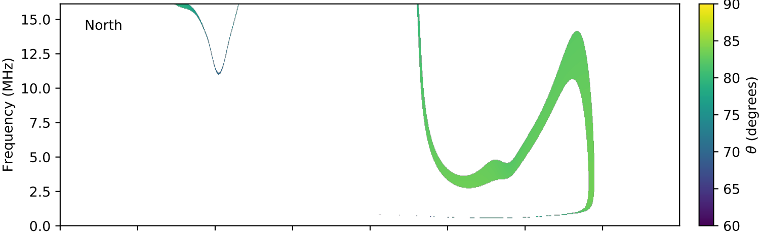
expres_cassini_jupiter_europa_isaac_lossc-wid1deg_3kev_20030220_v01.cdf
