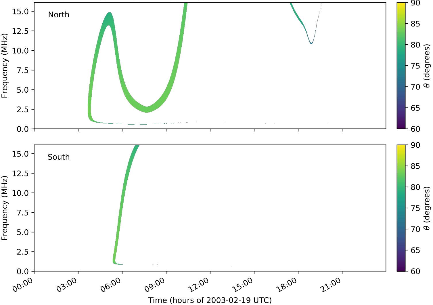
expres_cassini_jupiter_europa_isaac_lossc-wid1deg_3kev_20030219_v01.cdf
