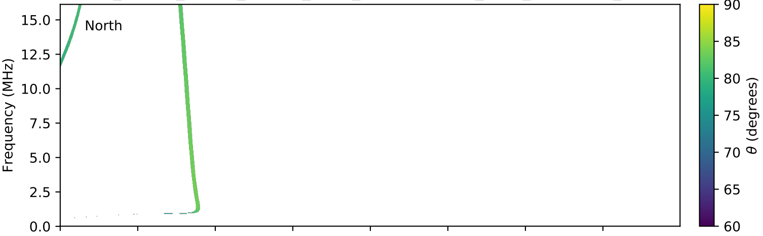
expres_cassini_jupiter_europa_isaac_lossc-wid1deg_3kev_20030217_v01.cdf
