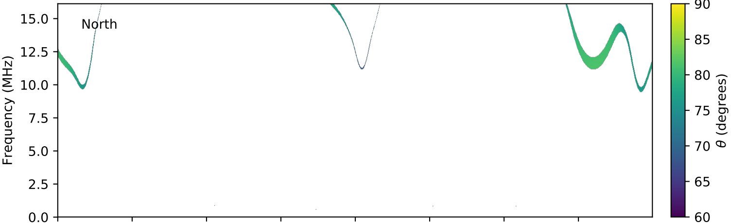
expres_cassini_jupiter_europa_isaac_lossc-wid1deg_3kev_20030216_v01.cdf
