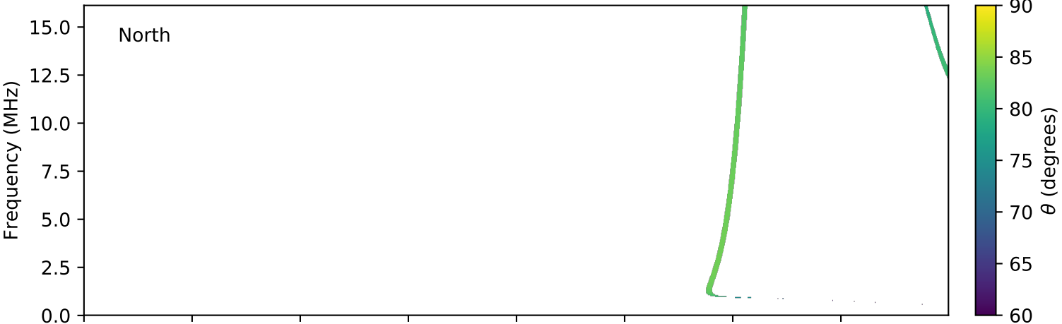
expres_cassini_jupiter_europa_isaac_lossc-wid1deg_3kev_20030215_v01.cdf
