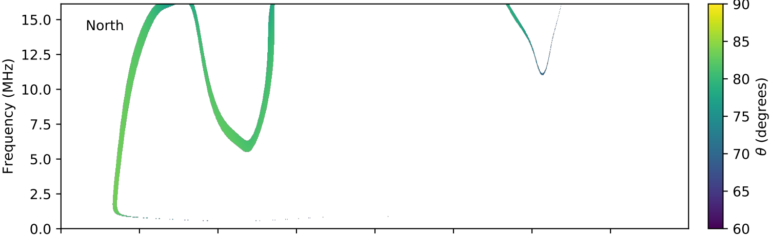
expres_cassini_jupiter_europa_isaac_lossc-wid1deg_3kev_20030212_v01.cdf
