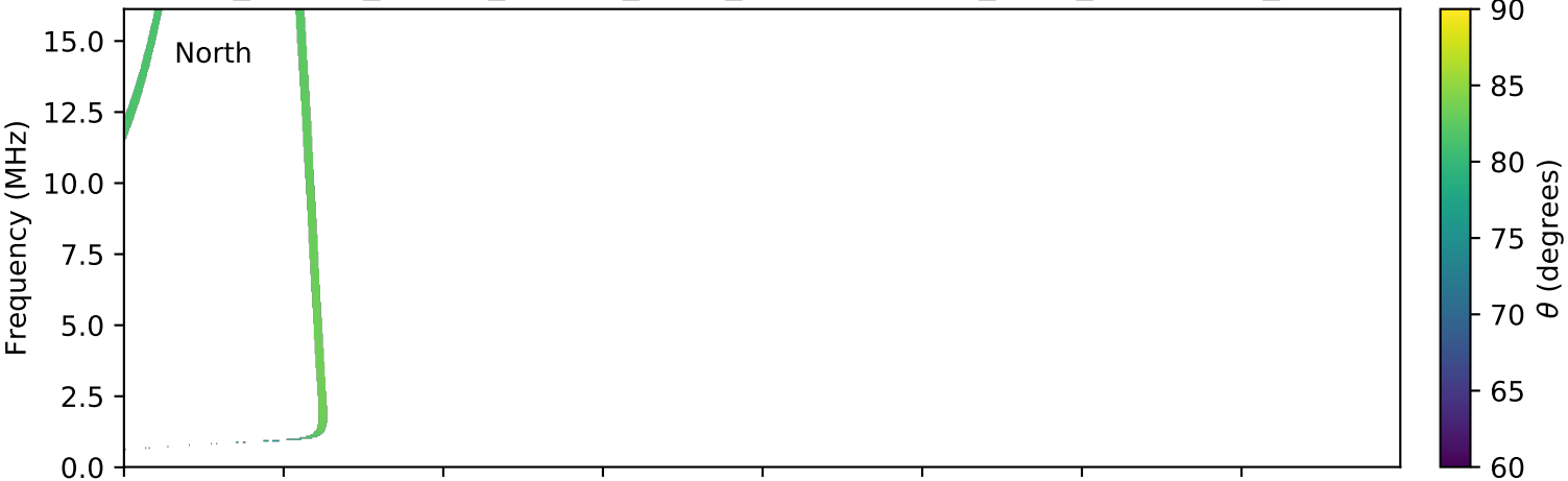
expres_cassini_jupiter_europa_isaac_lossc-wid1deg_3kev_20030210_v01.cdf
