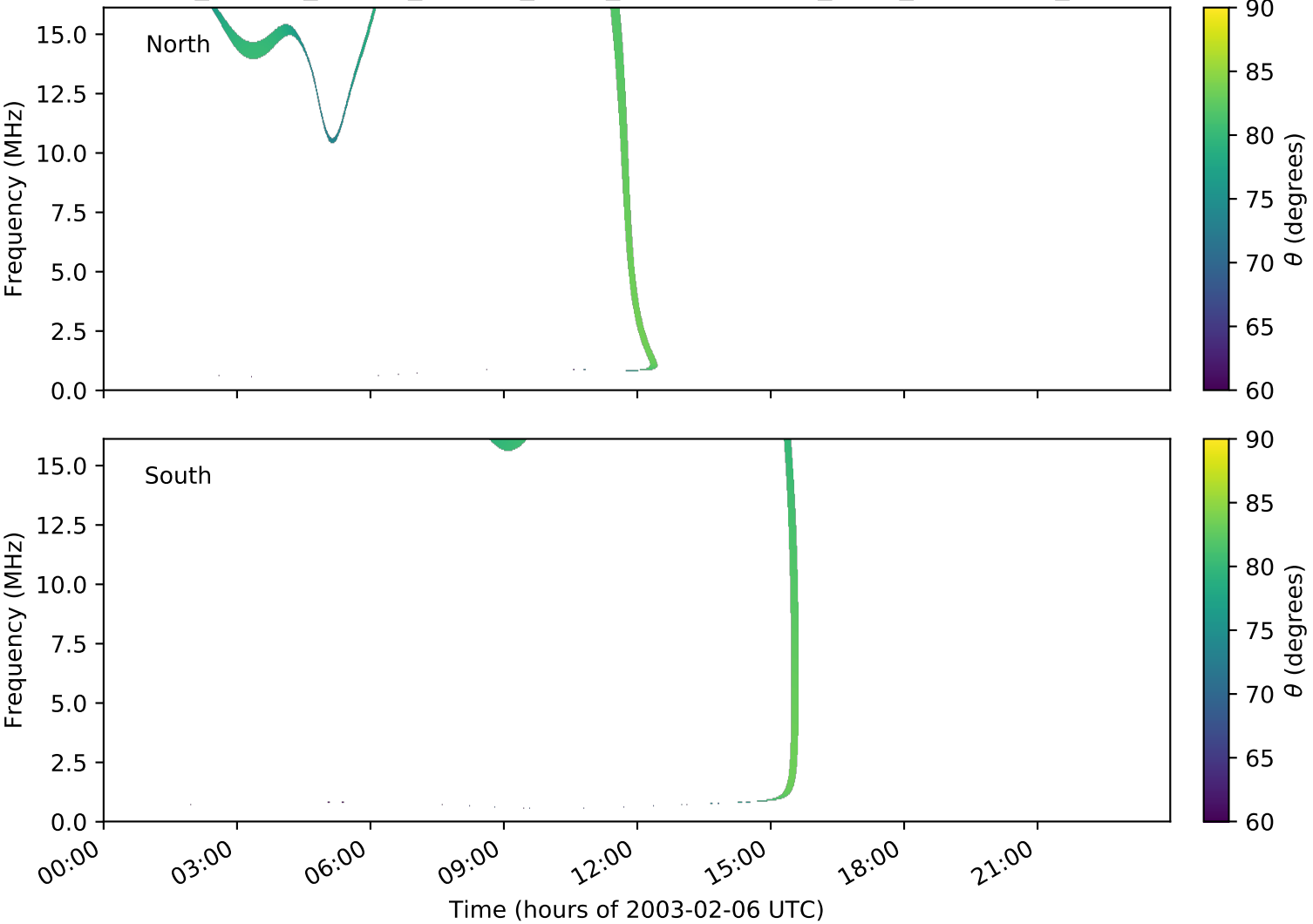
expres_cassini_jupiter_europa_isaac_lossc-wid1deg_3kev_20030206_v01.cdf
