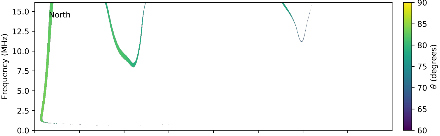
expres_cassini_jupiter_europa_isaac_lossc-wid1deg_3kev_20030205_v01.cdf
