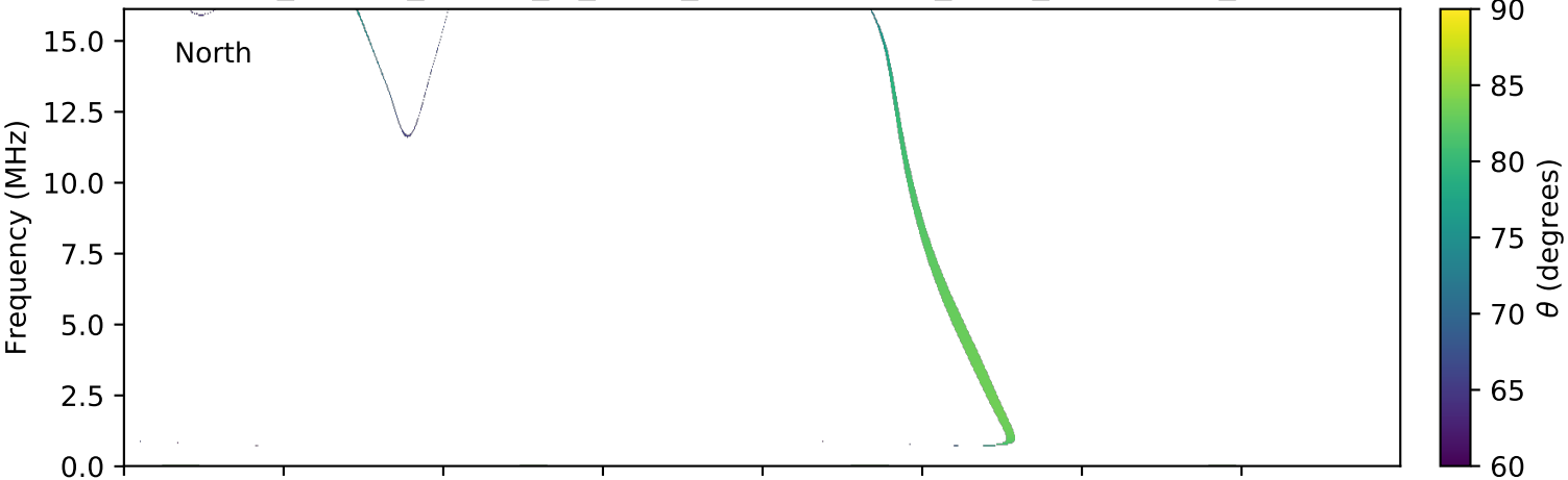
expres_cassini_jupiter_io_isaac_lossc-wid1deg_3kev_20030127_v01.cdf
