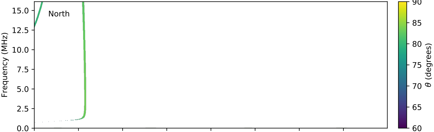
expres_cassini_jupiter_io_isaac_lossc-wid1deg_3kev_20030117_v01.cdf
