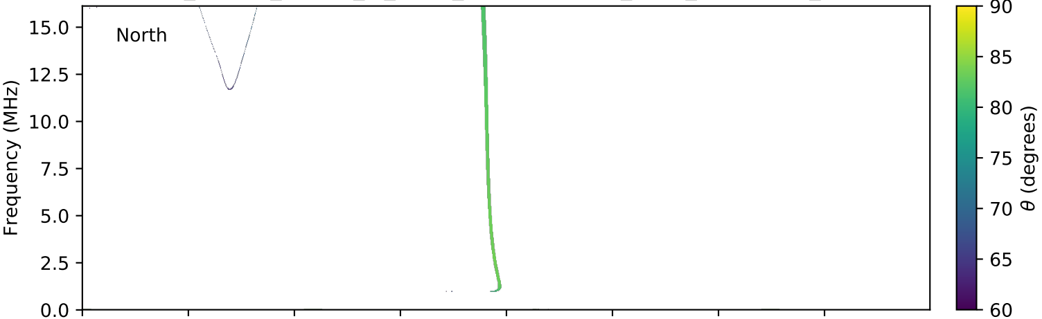
expres_cassini_jupiter_io_isaac_lossc-wid1deg_3kev_20030106_v01.cdf
