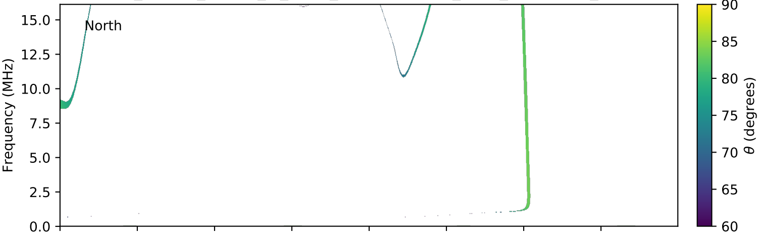
expres_cassini_jupiter_io_isaac_lossc-wid1deg_3kev_20030104_v01.cdf
