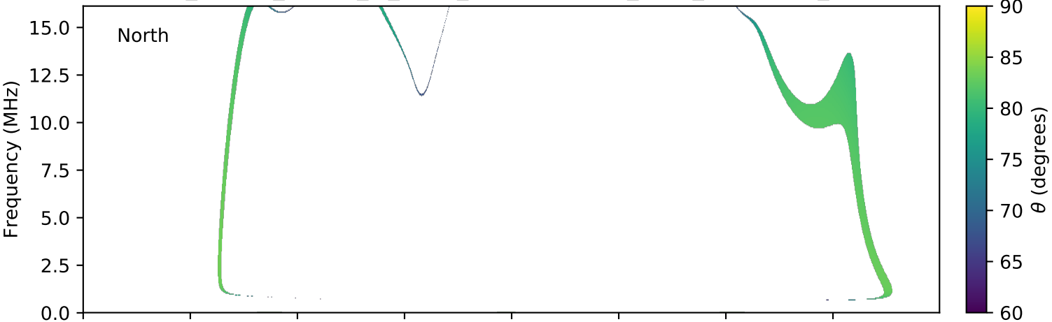
expres_cassini_jupiter_io_isaac_lossc-wid1deg_3kev_20030102_v01.cdf
