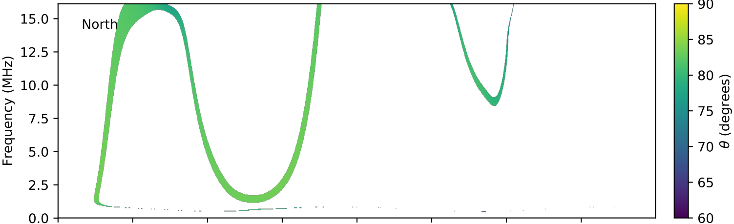
expres_cassini_jupiter_ganymede_isaac_lossc-wid1deg_3kev_20030131_v01.cdf
