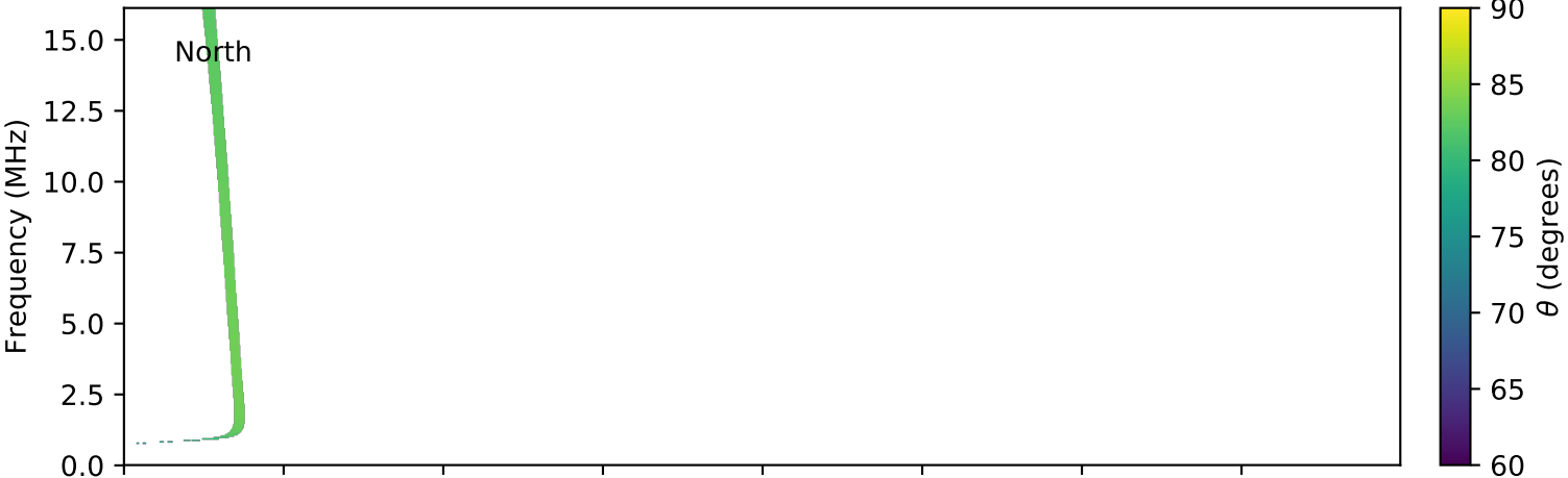
expres_cassini_jupiter_ganymede_isaac_lossc-wid1deg_3kev_20030127_v01.cdf
