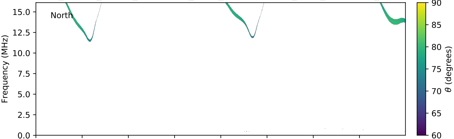
expres_cassini_jupiter_ganymede_isaac_lossc-wid1deg_3kev_20030125_v01.cdf
