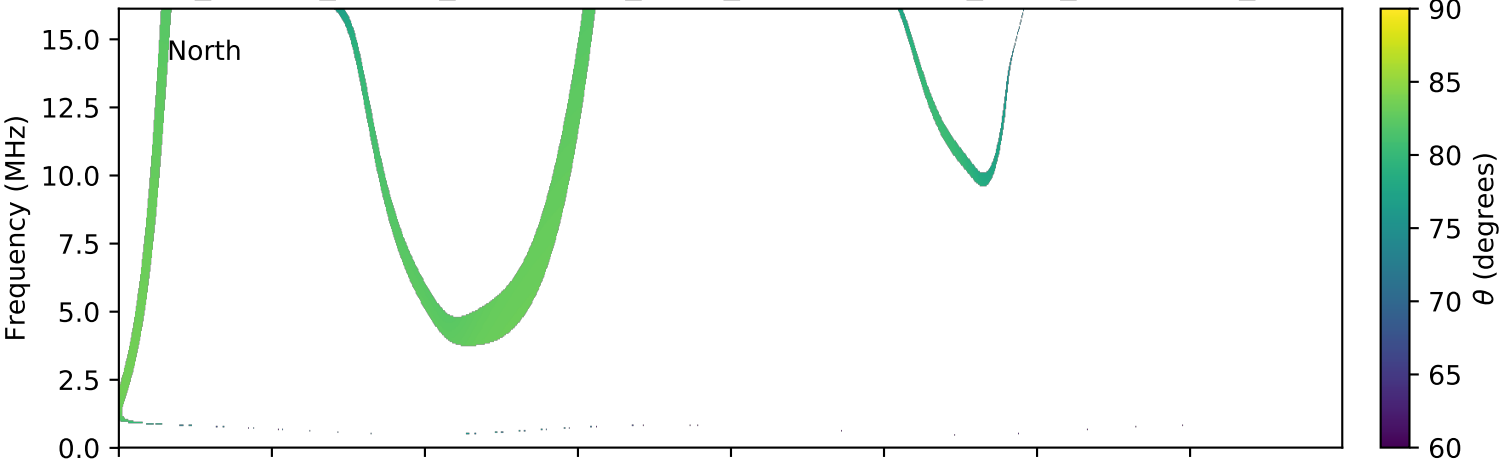
expres_cassini_jupiter_ganymede_isaac_lossc-wid1deg_3kev_20030124_v01.cdf
