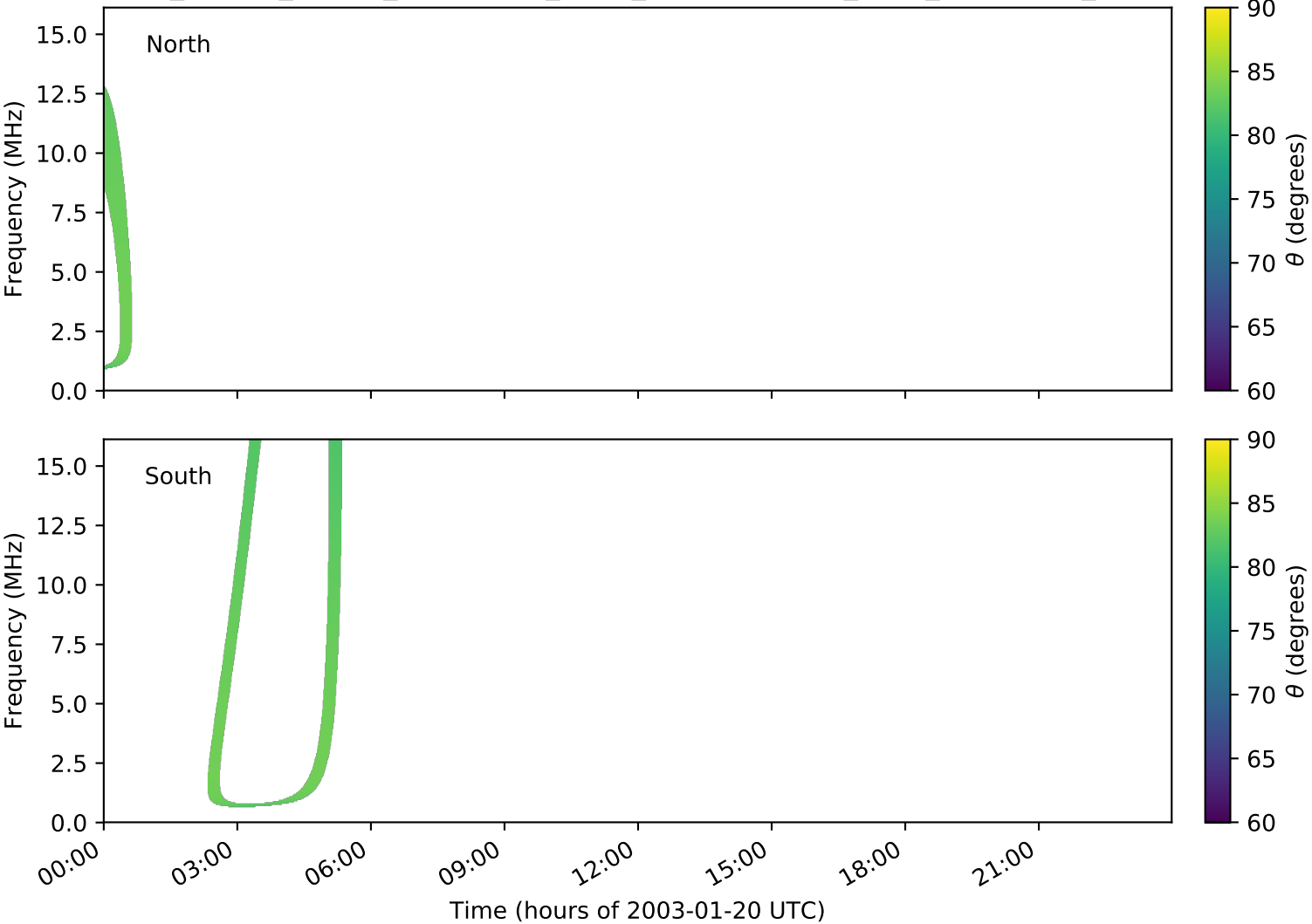
expres_cassini_jupiter_ganymede_isaac_lossc-wid1deg_3kev_20030120_v01.cdf
