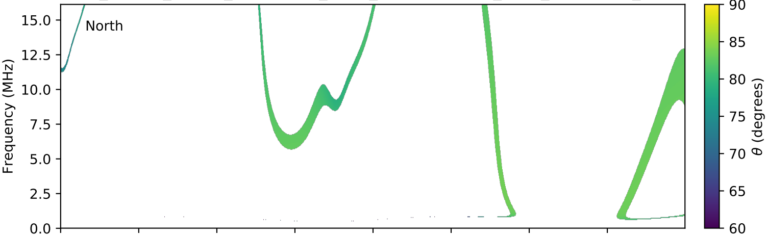
expres_cassini_jupiter_ganymede_isaac_lossc-wid1deg_3kev_20030119_v01.cdf
