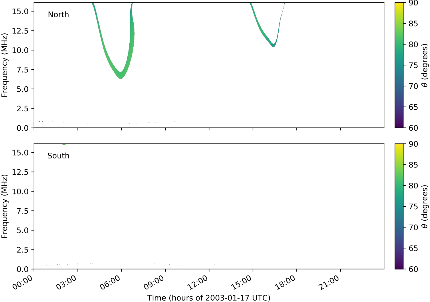
expres_cassini_jupiter_ganymede_isaac_lossc-wid1deg_3kev_20030117_v01.cdf
