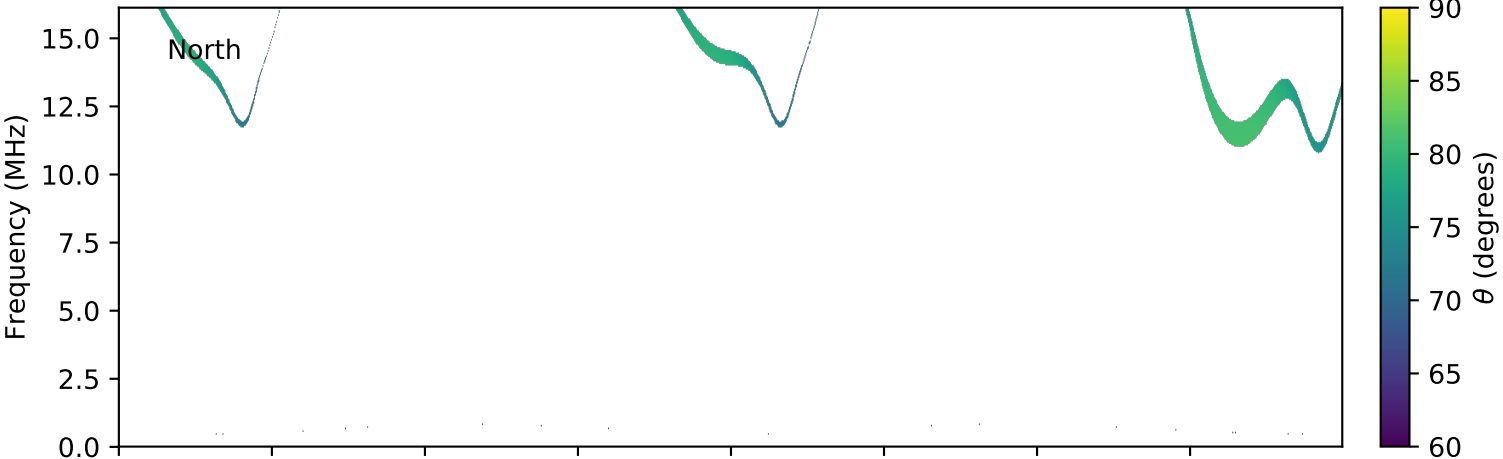
expres_cassini_jupiter_ganymede_isaac_lossc-wid1deg_3kev_20030111_v01.cdf
