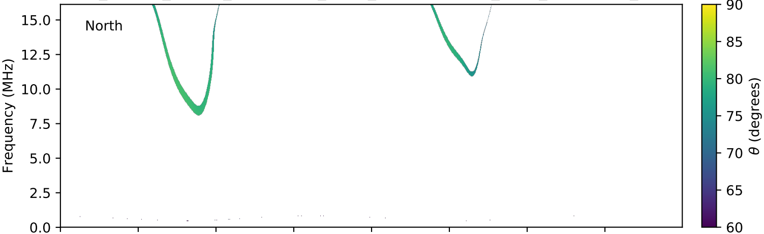
expres_cassini_jupiter_ganymede_isaac_lossc-wid1deg_3kev_20030110_v01.cdf
