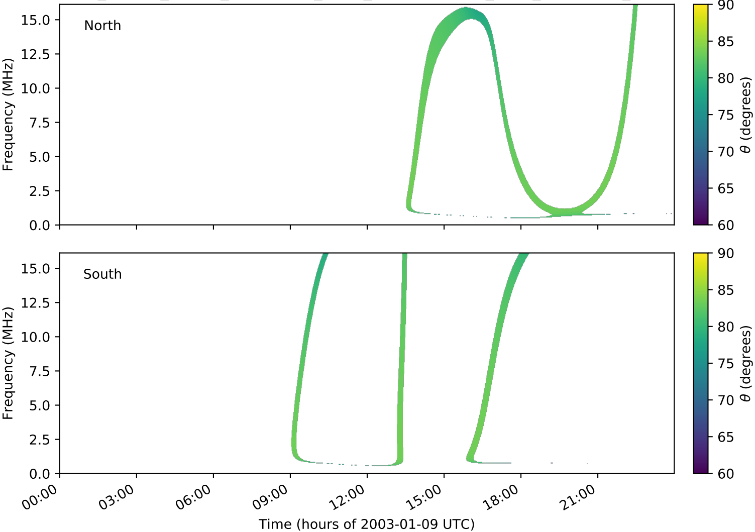
expres_cassini_jupiter_ganymede_isaac_lossc-wid1deg_3kev_20030109_v01.cdf
