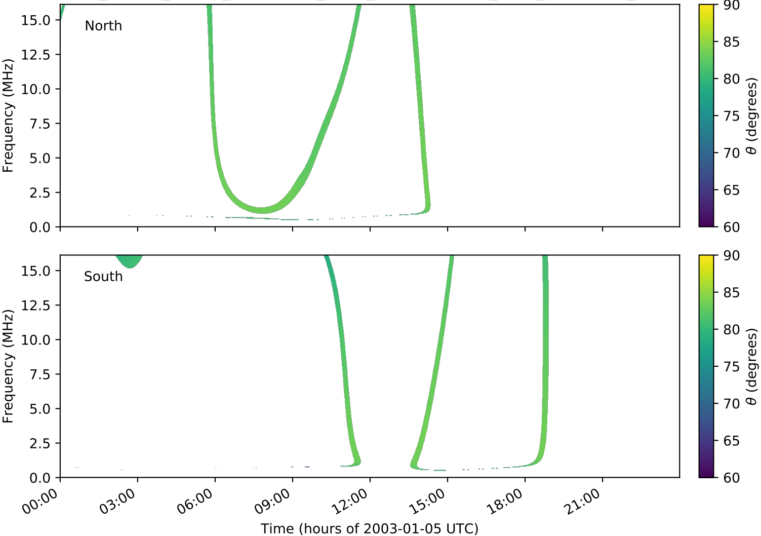
expres_cassini_jupiter_ganymede_isaac_lossc-wid1deg_3kev_20030105_v01.cdf
