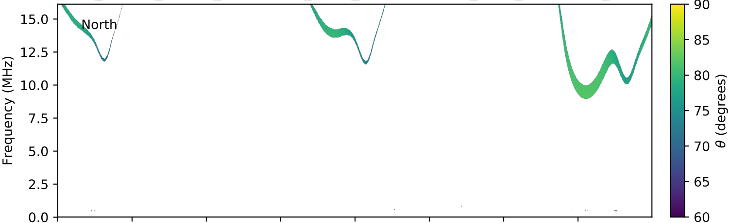
expres_cassini_jupiter_ganymede_isaac_lossc-wid1deg_3kev_20030104_v01.cdf
