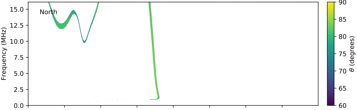
expres_cassini_jupiter_europa_isaac_lossc-wid1deg_3kev_20030130_v01.cdf
