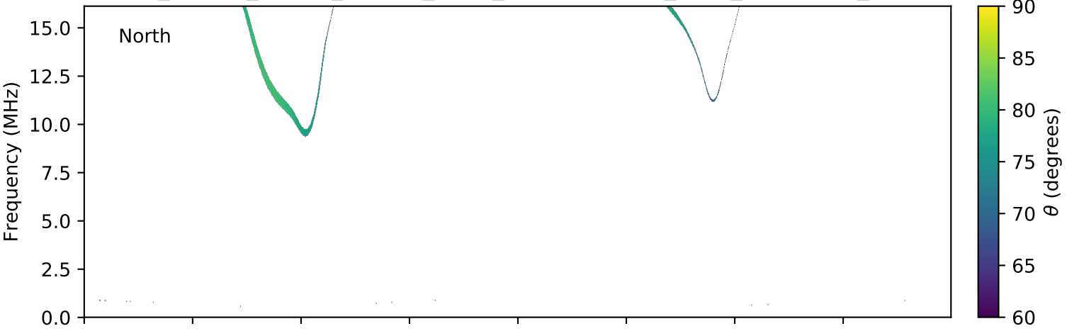
expres_cassini_jupiter_europa_isaac_lossc-wid1deg_3kev_20030129_v01.cdf
