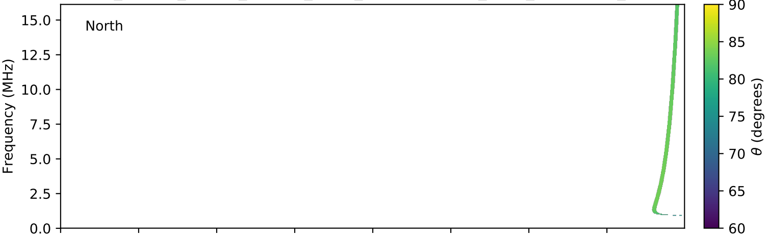
expres_cassini_jupiter_europa_isaac_lossc-wid1deg_3kev_20030128_v01.cdf
