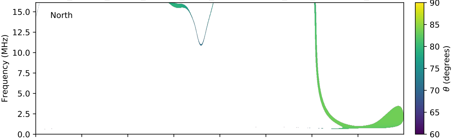
expres_cassini_jupiter_europa_isaac_lossc-wid1deg_3kev_20030126_v01.cdf
