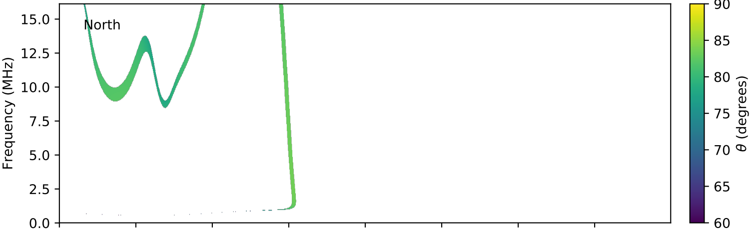
expres_cassini_jupiter_europa_isaac_lossc-wid1deg_3kev_20030123_v01.cdf
