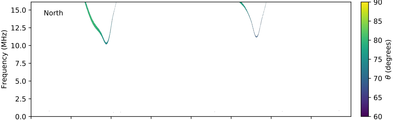
expres_cassini_jupiter_europa_isaac_lossc-wid1deg_3kev_20030122_v01.cdf
