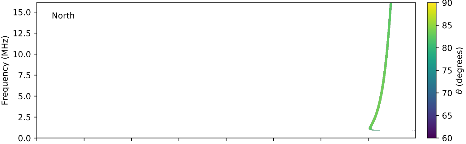
expres_cassini_jupiter_europa_isaac_lossc-wid1deg_3kev_20030121_v01.cdf
