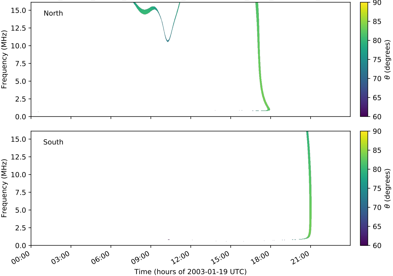
expres_cassini_jupiter_europa_isaac_lossc-wid1deg_3kev_20030119_v01.cdf
