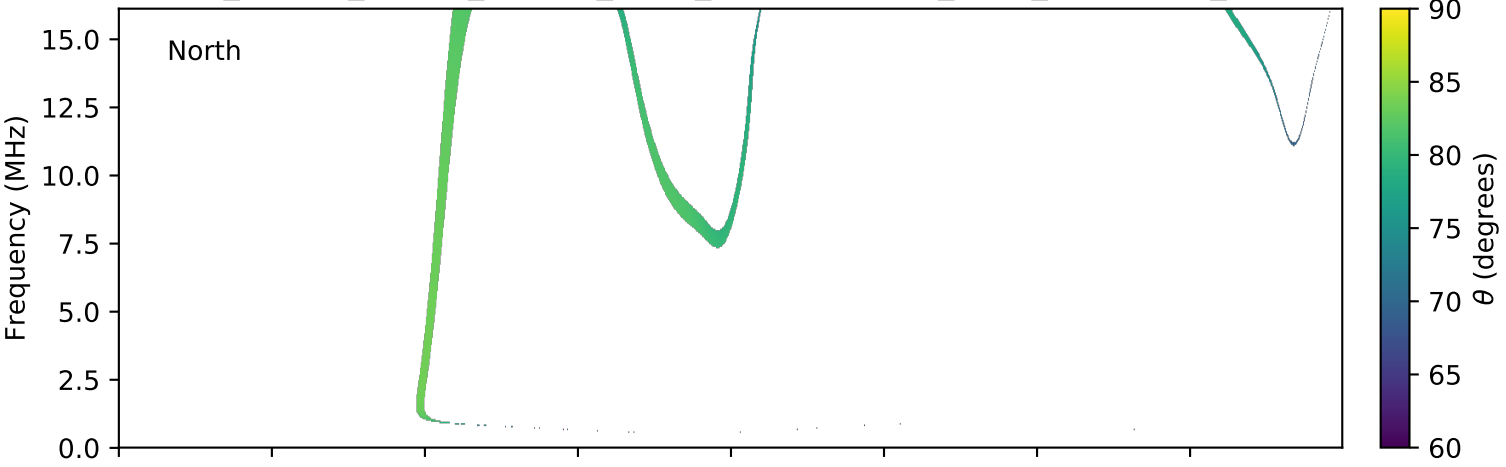
expres_cassini_jupiter_europa_isaac_lossc-wid1deg_3kev_20030118_v01.cdf
