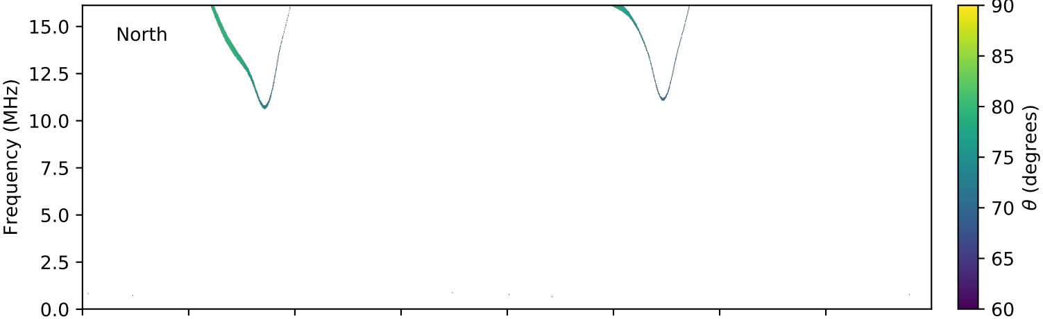
expres_cassini_jupiter_europa_isaac_lossc-wid1deg_3kev_20030115_v01.cdf
