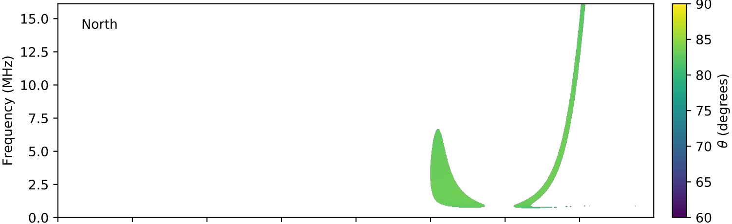
expres_cassini_jupiter_europa_isaac_lossc-wid1deg_3kev_20030114_v01.cdf
