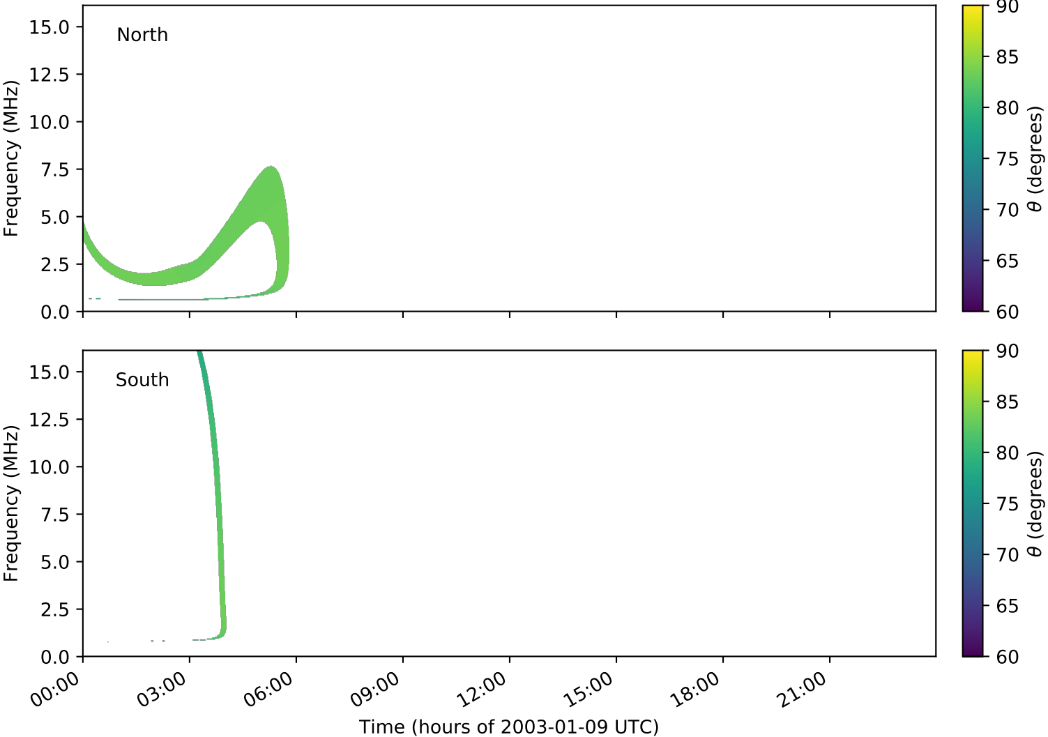
expres_cassini_jupiter_europa_isaac_lossc-wid1deg_3kev_20030109_v01.cdf
