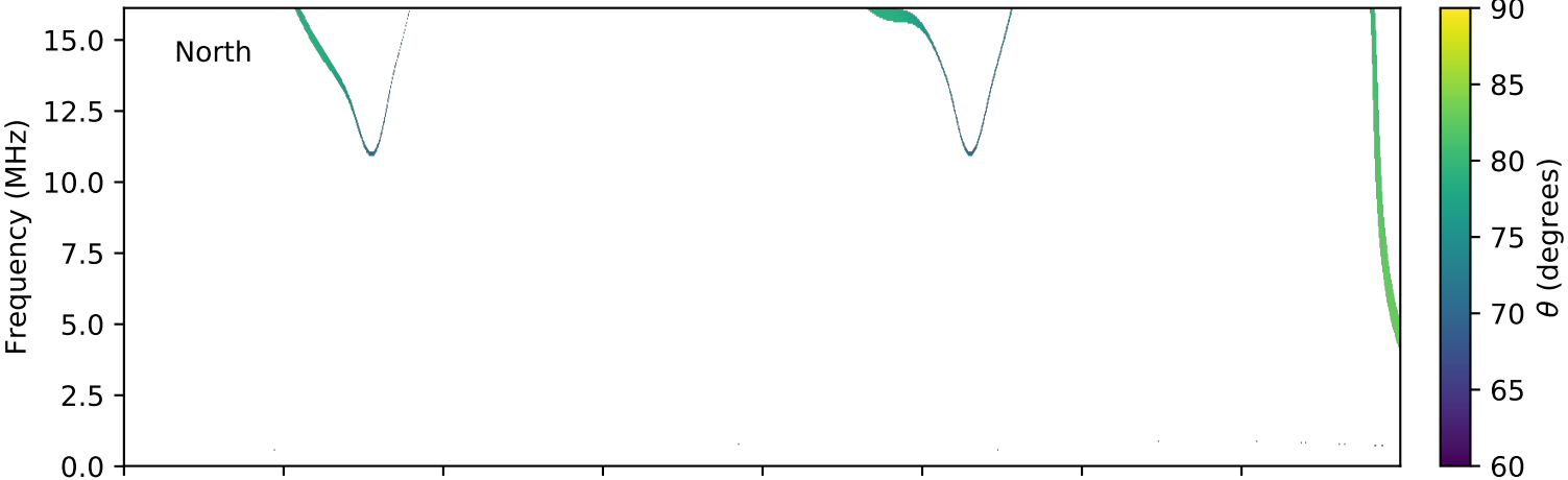
expres_cassini_jupiter_europa_isaac_lossc-wid1deg_3kev_20030108_v01.cdf
