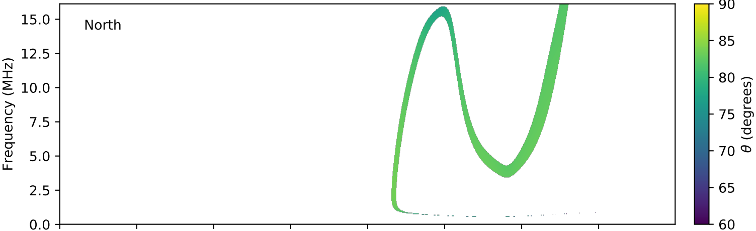
expres_cassini_jupiter_europa_isaac_lossc-wid1deg_3kev_20030107_v01.cdf
