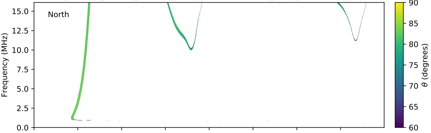
expres_cassini_jupiter_europa_isaac_lossc-wid1deg_3kev_20030104_v01.cdf
