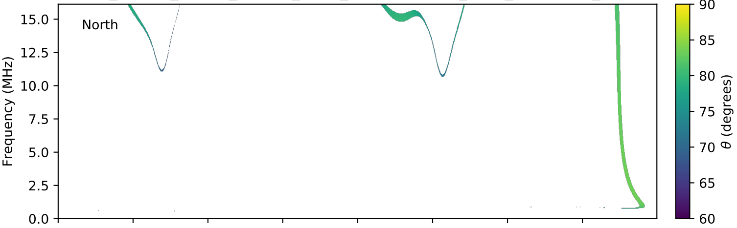
expres_cassini_jupiter_europa_isaac_lossc-wid1deg_3kev_20030101_v01.cdf
