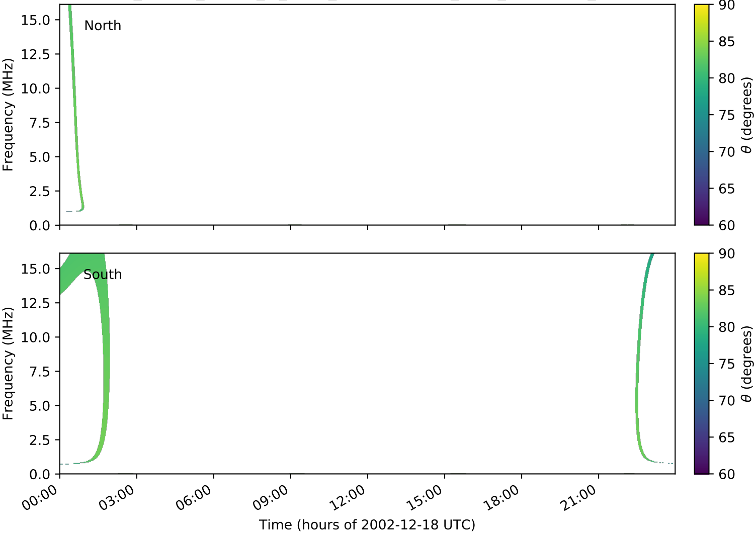
expres_cassini_jupiter_io_isaac_lossc-wid1deg_3kev_20021218_v01.cdf
