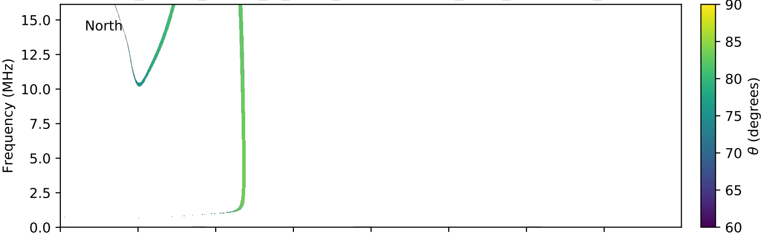
expres_cassini_jupiter_io_isaac_lossc-wid1deg_3kev_20021216_v01.cdf
