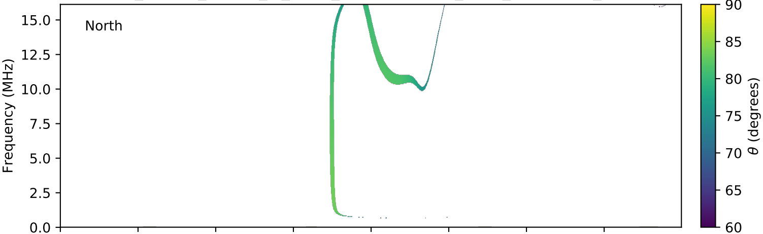
expres_cassini_jupiter_io_isaac_lossc-wid1deg_3kev_20021215_v01.cdf
