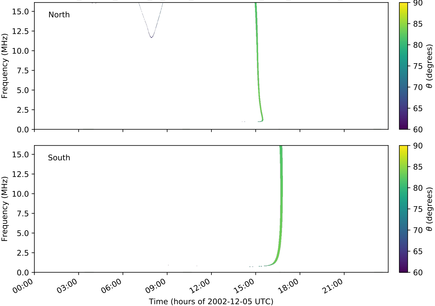
expres_cassini_jupiter_io_isaac_lossc-wid1deg_3kev_20021205_v01.cdf
