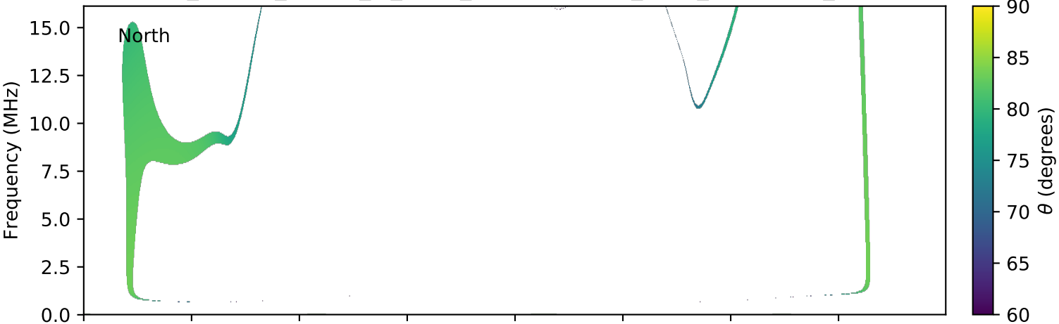
expres_cassini_jupiter_io_isaac_lossc-wid1deg_3kev_20021203_v01.cdf
