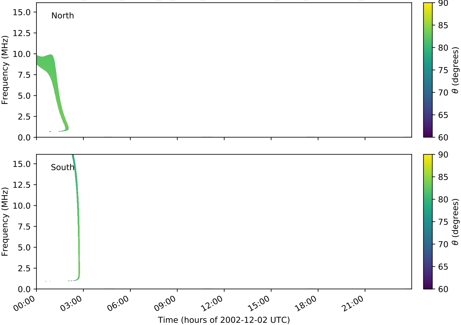
expres_cassini_jupiter_io_isaac_lossc-wid1deg_3kev_20021202_v01.cdf
