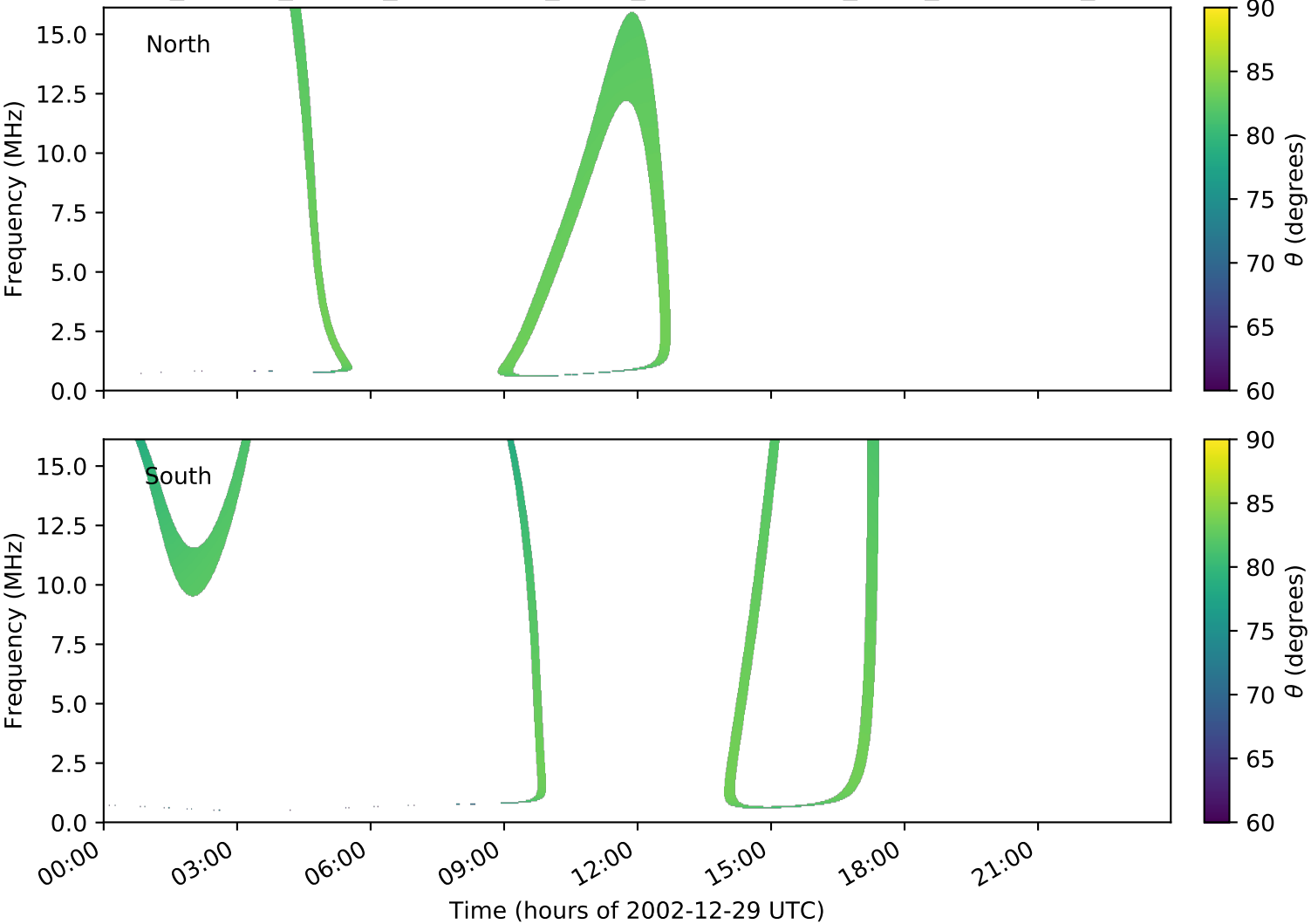
expres_cassini_jupiter_ganymede_isaac_lossc-wid1deg_3kev_20021229_v01.cdf
