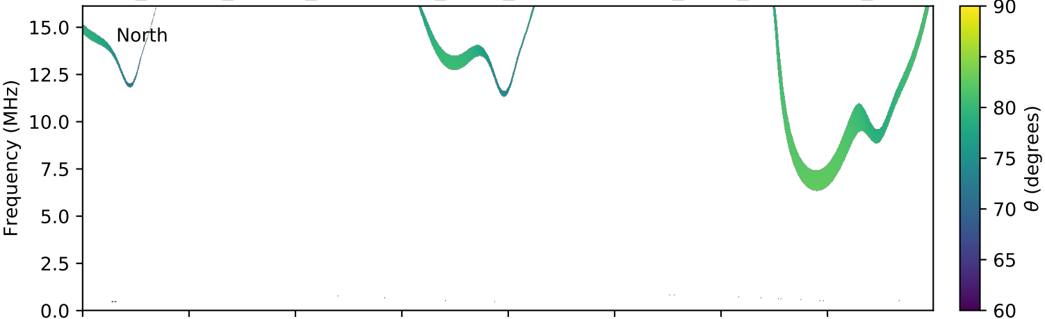
expres_cassini_jupiter_ganymede_isaac_lossc-wid1deg_3kev_20021228_v01.cdf
